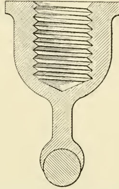
Fig. 185. Section of Ear with Trolley Wire Soldered in Place
